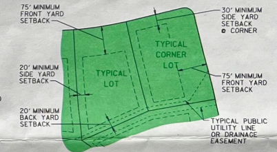
TYPICAL LOT LAYOUTS
